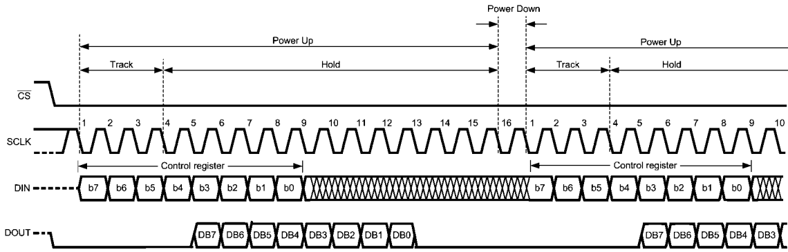
ADC084S051 Operational Timing Diagram
